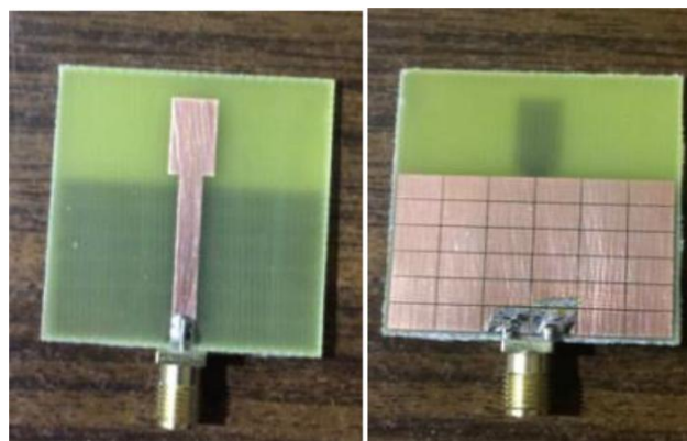
(a) (b) Figure 12 Fabricated Antenna a) Top View b) Bottom View
