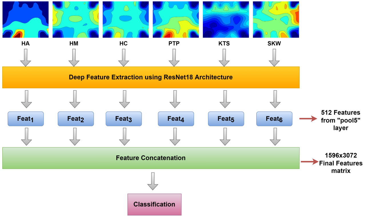
Fig. 2: Flowchart illustrating the procedures for extracting, fusing, and classifying deep features.
