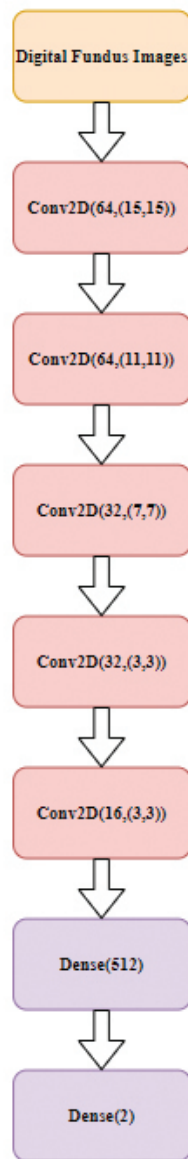
Figure 3. Proposed two-dimensional convolutional neural network architecture (Conv2D [neuron number, filter size] and Dense [neuron number])
