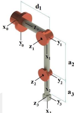
Figure 1. 3 DOF robot manipulator.
